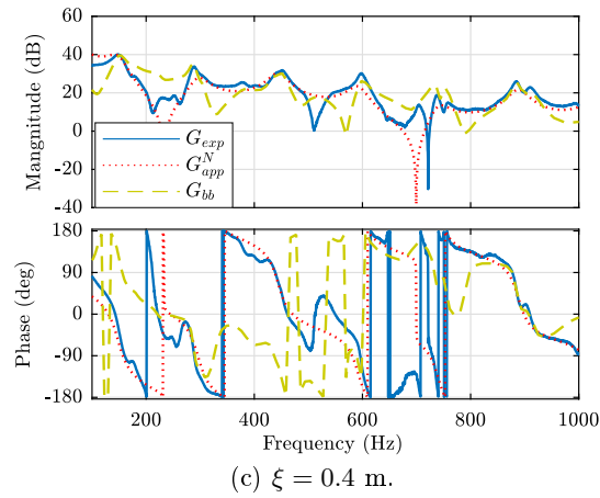
Figure 6: Experimental frequency responses ( y = 0.125 m, z = 0.15 m).
