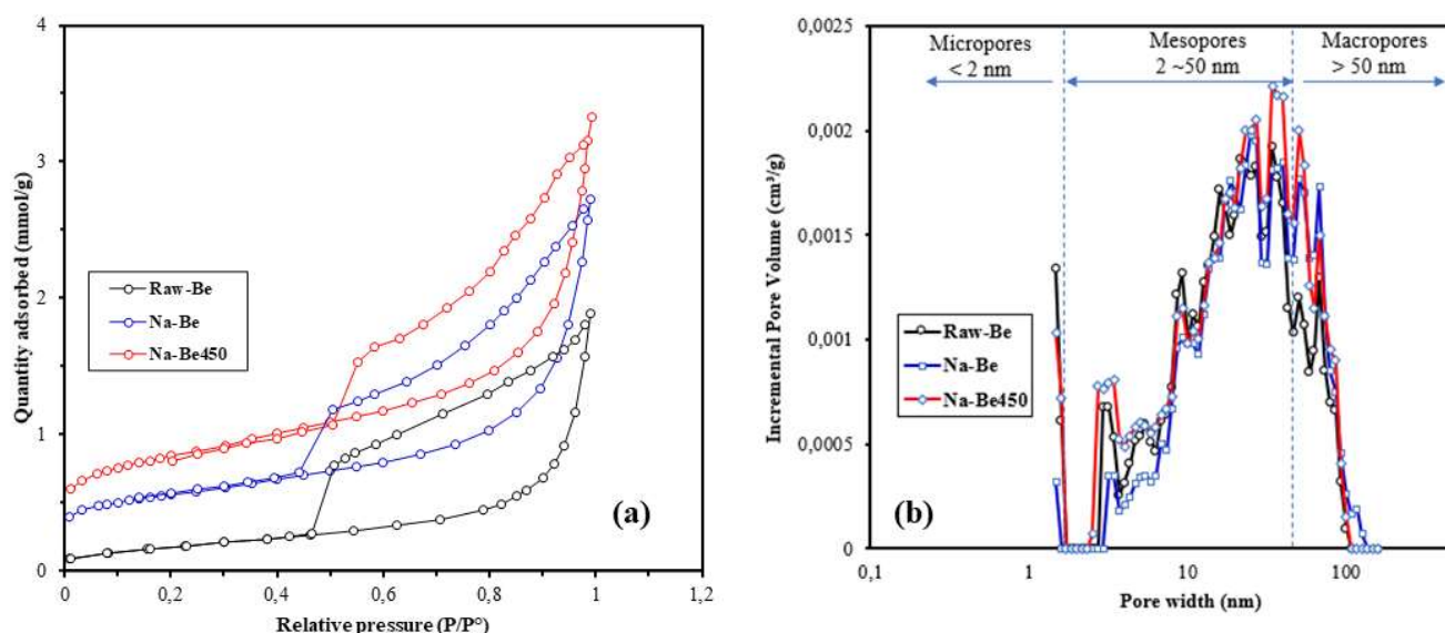
Fig.4. Nitrogen adsorption-desorption isotherms (a) and pore size distributions (b) for modified bentonites Raw-Be, Na-Be and Na-Be450.
