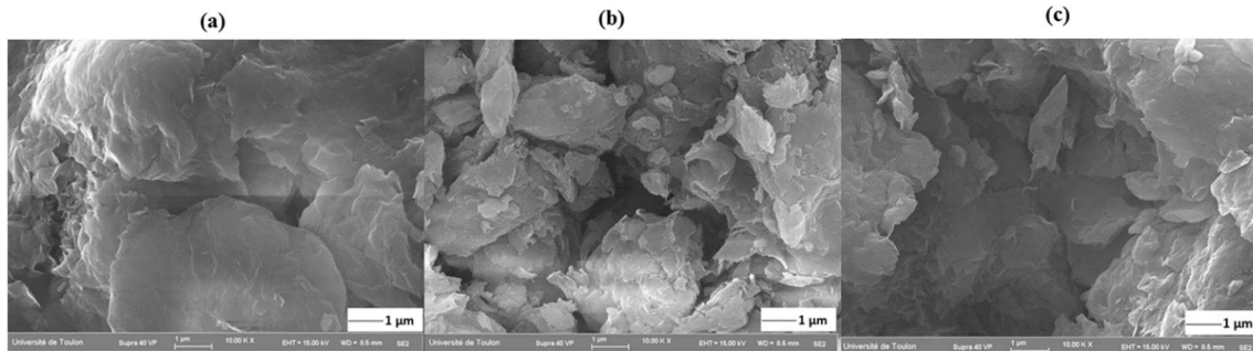
Fig.3. SEM images of Raw-Be (a), Na-Be (b) and Na-Be450 (c).
