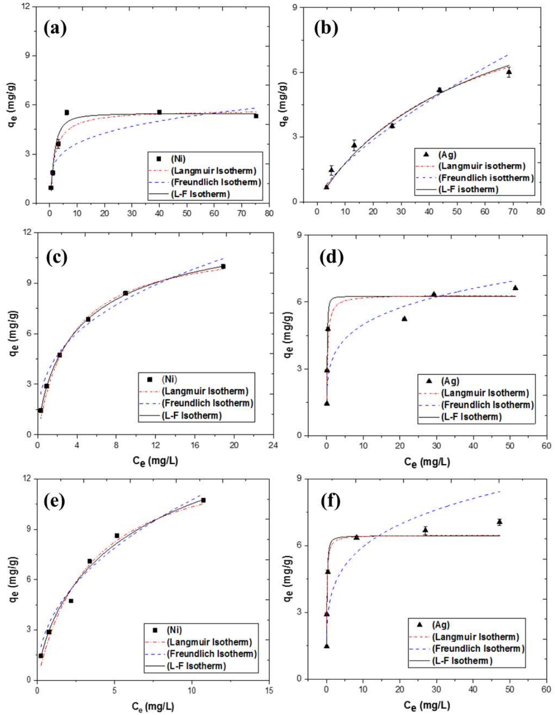
Fig.6. Equilibrium isotherms for Ni adsorption onto (a) Raw-Be (c) Na-Be and (e) Na-Be450 as well as equilibrium isotherms for Ag adsorption onto (b) Raw-Be (d) Na-Be and (f) Na-Be450. Dotted, dash-dotted and solid lines represent Langmuir fitting, Freundlich and Langmuir-Freundlich fitting, respectively.
