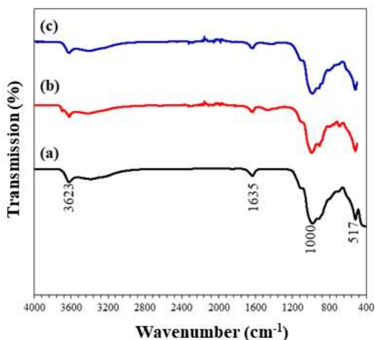
Fig.2. FTIR spectra of raw-Be (a), Na-Be (b) and Na-Be450 (c).
