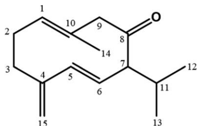
Figure 6: Atomic structure of germacrene D-8-one
