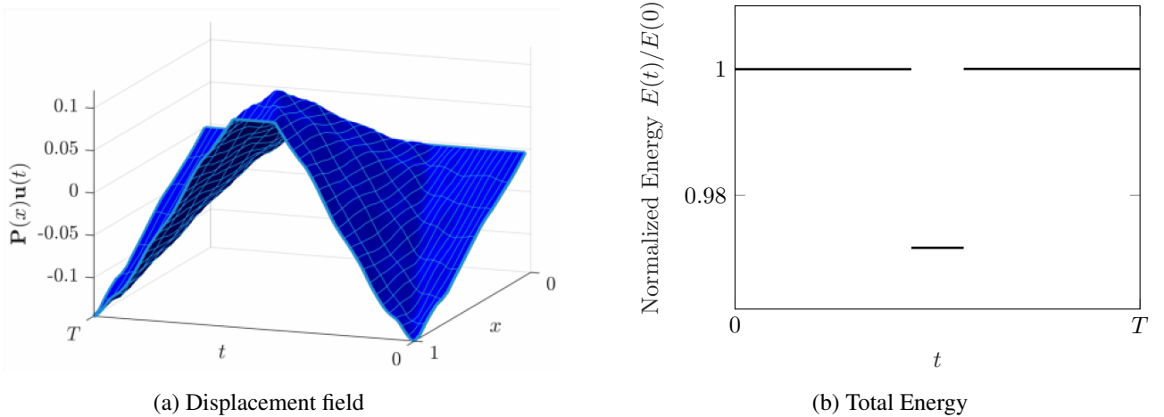
Figure 3: NBM periodic solution for the varying area bar (corresponding to the model investigated in Figure 4) of 10 elements and quadratic Lagrangian shape functions ( N = 20 ). Note that the total energy is dissipated at the moment of contact but is completely regained at the end of the contact phase. Due to this characteristic, the NBM allows for periodic solutions with sticking phases.
