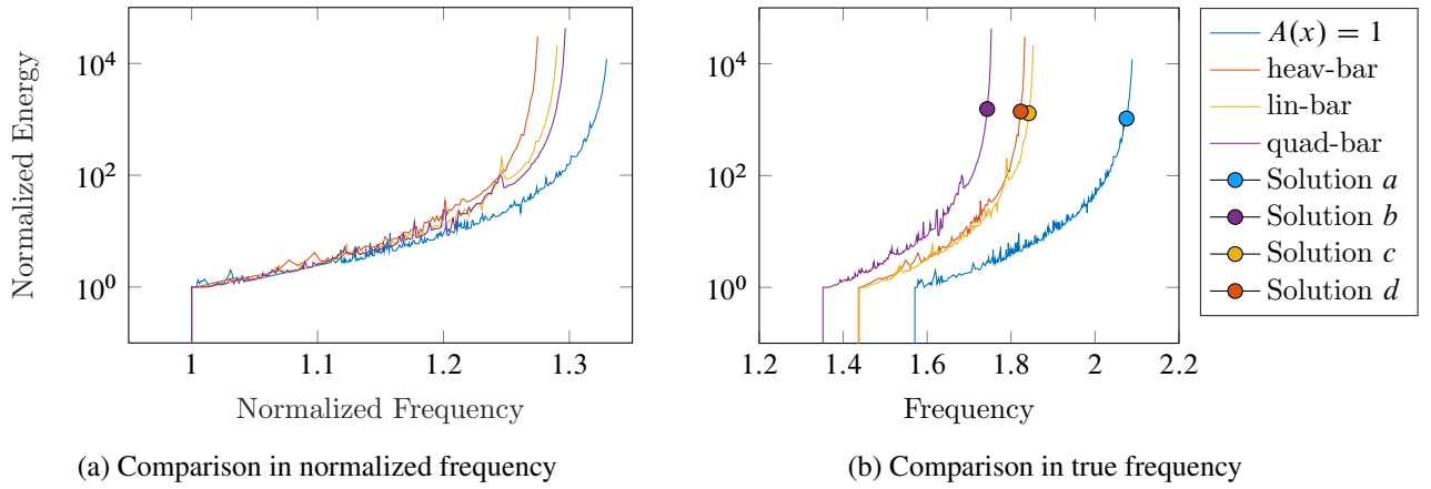
Figure 11: Backbone curves of different area cantilever bars corresponding to Figure 8(a) and Figure 10.
