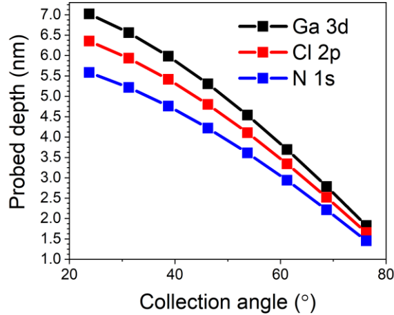
Fig. 3. Ga 3d, Cl 2p and N 1s probed depths as a function of the collection angle.
