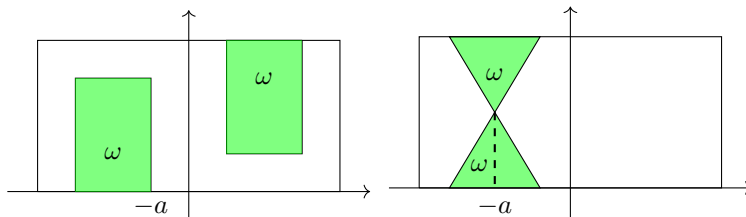
FIGURE 5. In these configurations, we obtain a lower bound on the critical time of null-controllability.
