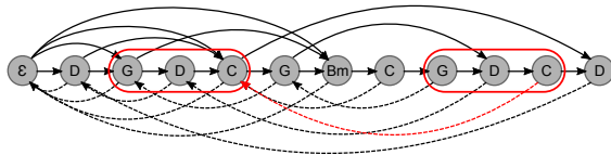
Figure 2. Factor oracle created from the chord progression D G D C G Bm C G D C D. Curved arrows at the upper half are used during the construction of the oracle, but are not used anymore. Suffix links (dashed arrows) connect each state to the past states sharing the longest common context. The two states connected by the bold suffix link share the common context G D C. A possible generation by navigating the oracle is D G D C * D . G, taking this suffix link towards the future (*), then, after the last state D, taking a suffix link towards the past. This generation was not present in the original chord progression but nevertheless share significant sub-progressions with it.
