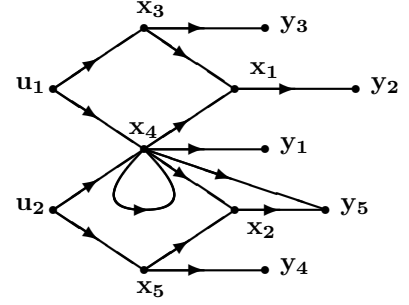
FIGURE 4. Digraph of Example 2
