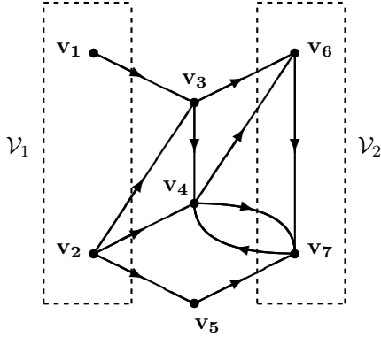
FIGURE 1. Example of digraph
