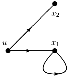
FIGURE 2. Digraph of Example 1.1
