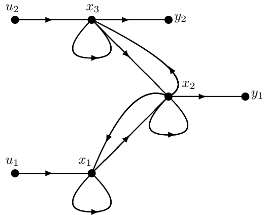
FIGURE 3. Digraph of Example 1.2
