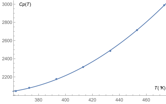
FIG. 2. Graph associated with experimental Table I and Eq. (35). The x axis indicates the Kelvin temperature, and the y axis indicates for water the corresponding isobaric heat capacity c_p expressed in J\ kg^{-1}\ K^{-1} . The dots represent c_p values coming from experimental Table I.
