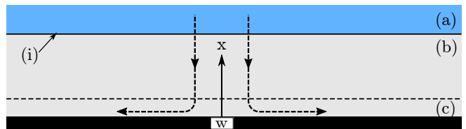
FIG. 1. Sketch of a quasi-one-dimensional transverse fluid flow. Domain (a) is a thin liquid layer; (i) is the liquid–vapor discontinuity interface which is a very thin region of few nanometers thickness of the temperature T_i ; domain (b) is the non-isothermal part of the vapor flow; the temperature increases from T_i to T_w . Region (c) is the part of the vapor region where the flow is not one–dimensional: the vapor escapes along the solid surface. The arrows show the flow direction.
