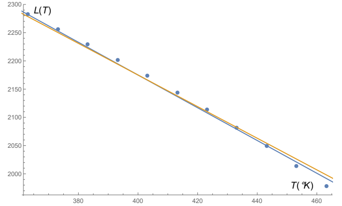
FIG. 3. The linear approximations of the latent heat of water in kJ\ kg^{-1} expressed by Eq. (36) (in yellow) and Eq. (37) (in blue) are shown as functions of the Kelvin temperature. The dots represent the values of L(T) from Table II.
