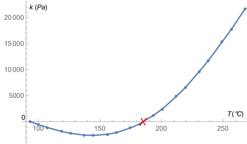
FIG. 4. Graphs associated with the k in Pa as a function of T^{\circ}\text{C} in the first linear approximation (36). The x axis is associated with the Celsius temperature and the y axis with the pressure k expressed in Pascal. The dots represented k values calculated with the software Mathematica TM . In this case, the Leidenfrost temperature highlighted by a red cross is T_L \approx 185^{\circ}\text{C} .
