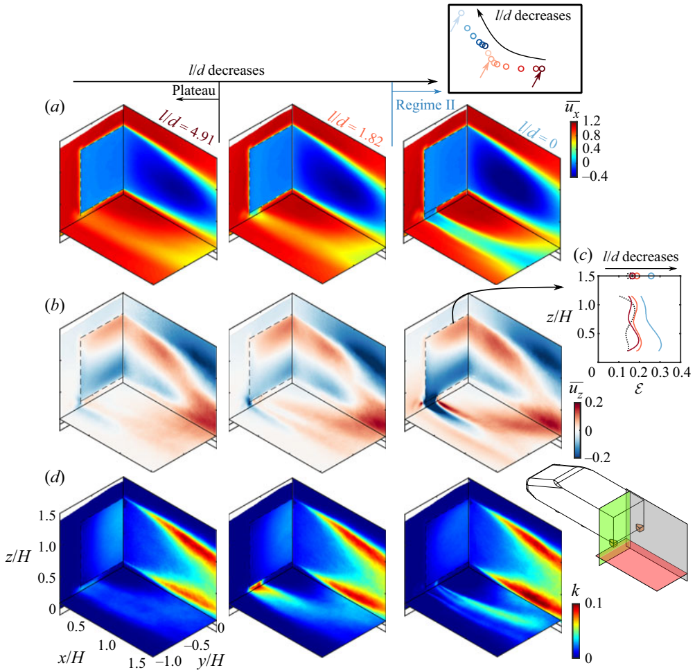
Figure 13. Mean velocity components, (a) \overline{u_x} and (b) \overline{u_z} , in the three PIV planes for the cases of the plateau ( l/d = 4.91 ), regime I ( l/d = 1.82 ) and regime II ( l/d = 0 ). The width of the obstacles is d_{ref}/H = 0.19 . (c) Comparison of the cross-flow strength \mathcal{E} , the space-averaged values are shown over the top axis. (d) Turbulent kinetic energy k distributions in the three PIV planes for the same cases as (a, b).
