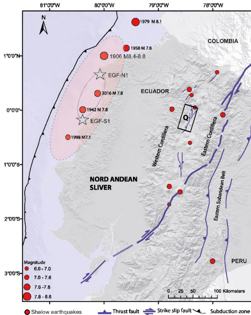
Figure 1. Ecuador main historical seismicity (Beauval et al. 2013) and tectonic settings. Red circles: epicentres of superficial earthquakes (depth < 50 km,) with M_w \geq 7.0 for subduction earthquakes and M_w \geq 6 for crustal earthquakes. Q indicates the location of the capital city of Ecuador, Quito. The light-red ellipsoids on the coast represent the approximate rupture area of the earthquakes simulated in this paper. The smallest correspond to the M_w 7.8 events and the largest to the M_w 8.5. They are there only to give an idea of the area that can be broken by the earthquakes, but this size strongly depends on the rupture parameters. The two stars represent the position of the earthquakes used as EGFs for the simulation of M_w < 8 events. Figure modified from Alvarado et al. (2014).
