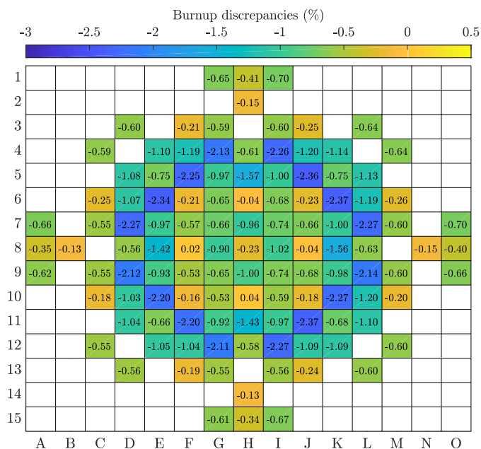
Fig. 7. Burnup discrepancies between predicted and calculated values at reloading.
