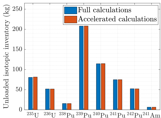
Fig. 8. Unloaded actinides inventories obtained with full and accelerated calculations.
