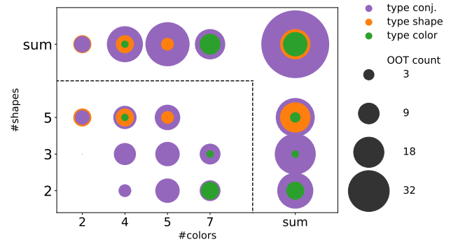
Figure 6: Number of trials for which the participants ran out of time (OOT) per type, #colors and #shapes. There are 116 OOT trials in total (5.5 per participant on average), 74% of which are of type conjunction, 16% are of type shape and 10% are of type color.
