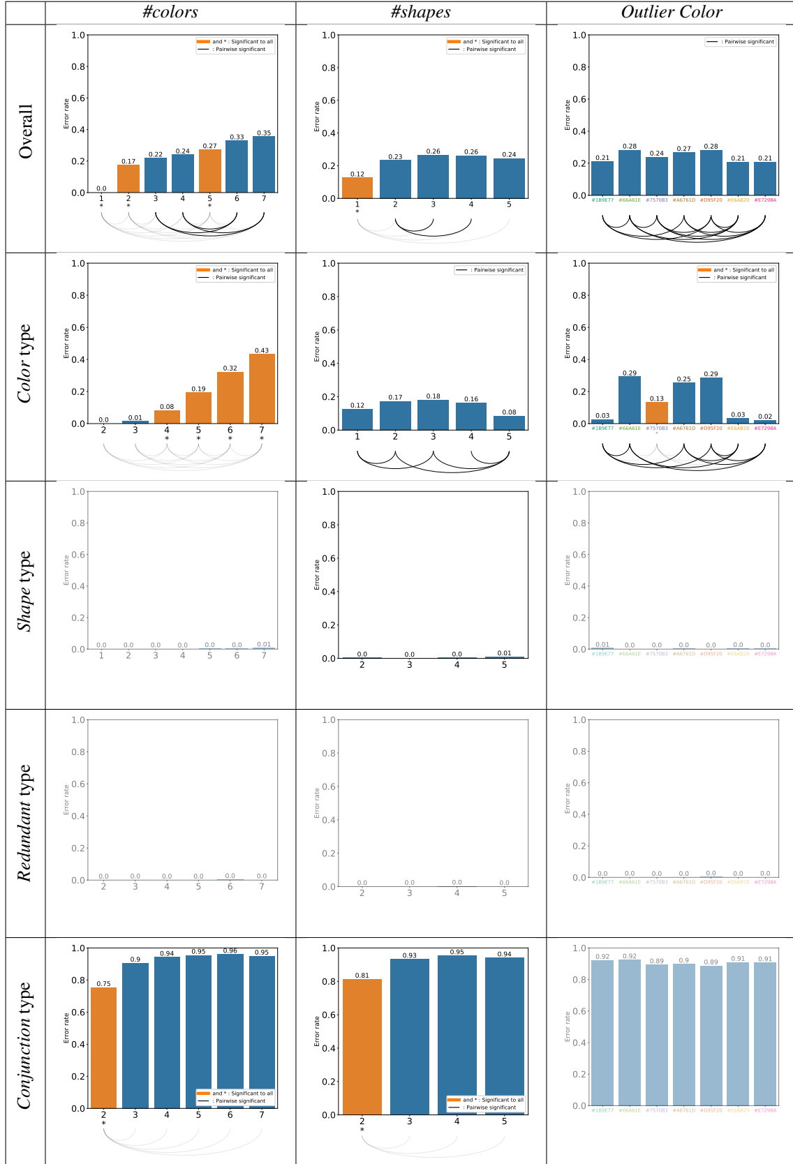
Figure 4: Trained ResNet error rates (ER) on the test set. The first row shows the overall parameters ERs, while the next rows present the parameters ERs by type . A plot is faded if the ANOVA test on its given parameter and type aggregation failed, meaning the parameter values variations did not have any significance effect on the condition; otherwise, it is opaque. An arc between two labels means that the pairwise comparison between the ERs of the two parameter values is significant according to a Wilcoxon rank-sum test. When performances associated to a label are significantly different to all others: the bar is colored orange and the symbol * is added below the label. The significance threshold was p\text{-value} < 0.05 for the ANOVA and pairwise tests in the overall studies, while it was p\text{-value} < 0.025 in the per type studies. A reading example is given in the caption of Figure 3.
