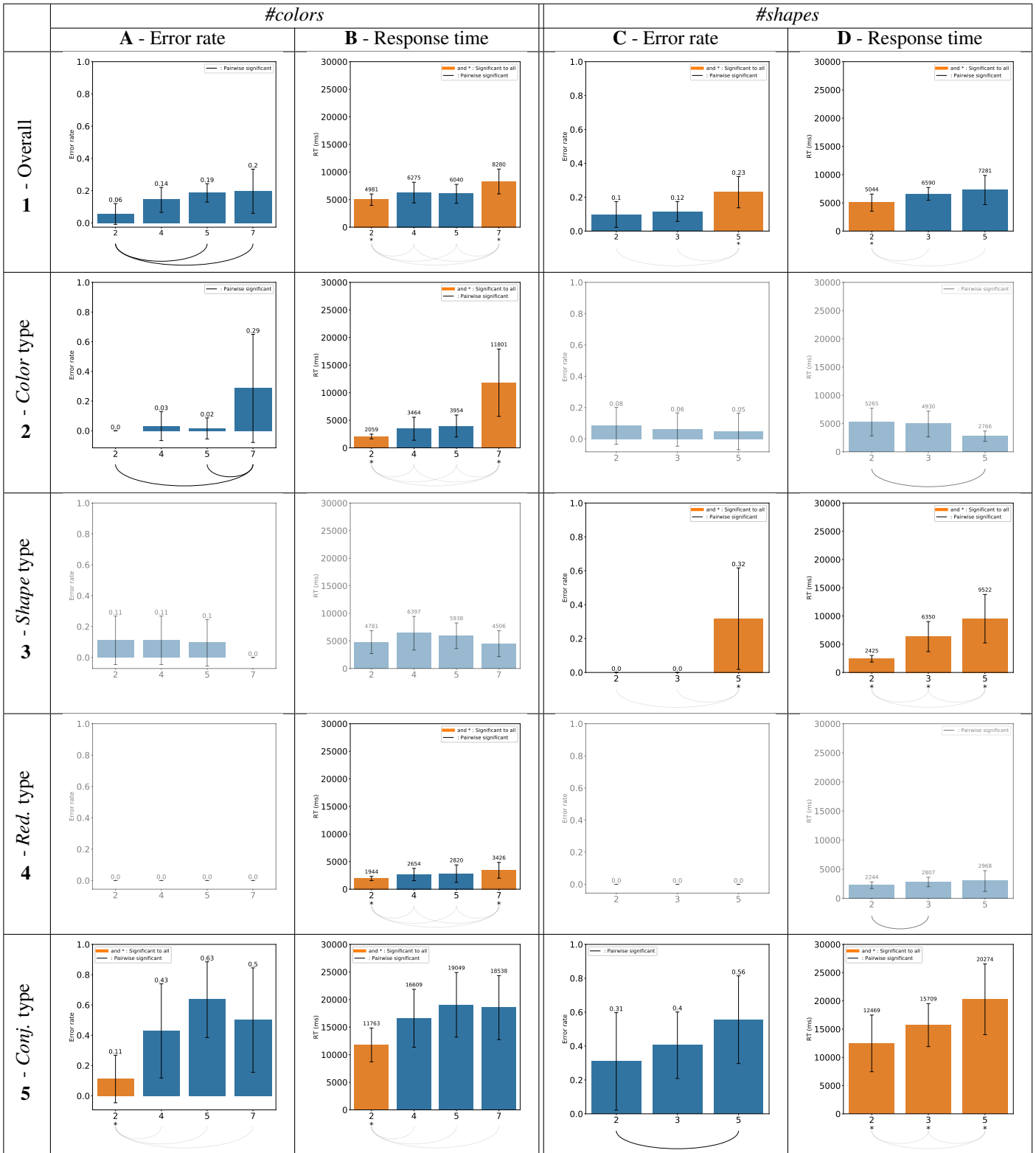
Figure 8: participants ERs and mean RTs with standard deviation bars measured during the evaluation. The first row shows the overall performances in terms of the parameter values, while the next rows present the parameter values achieved by type . A plot is faded if the ANOVA test on its given parameter and type aggregation failed; otherwise, it is opaque. An arc between two labels means that the pairwise comparison between the corresponding performance values is significant according to a Wilcoxon rank-sum test. When performances associated to a label are significantly different to all others: the bar is colored orange and the symbol * is added below the label. The significance threshold is p\text{-value} < 0.05 for the ANOVA and pairwise tests in Overall studies, while it is p\text{-value} < 0.025 in the per type studies. A reading example is given in the caption of Figure 7. In this table of plots, columns are given letters and rows are given numbers for ease of reference.
