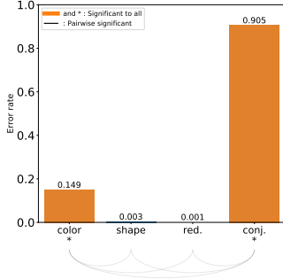
Figure 3: Trained ResNet error rates (ER) on the test set for the type values. An arc between two labels means that the pairwise comparison between the ER of the two parameter values is significant ( p -value < 0.05 ) according to a Wilcoxon rank-sum test. When performances associated to a label are significantly different to all others: the bar is colored orange and the symbol * is added below the label. Reading example: the color type is significantly easier than the conjunction type and significantly harder than the shape and redundant types. There is no significant difference between the redundant and shape types.
