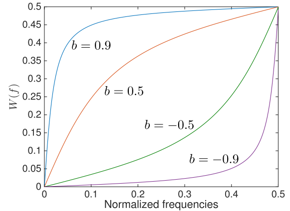
Fig. 3. Frequency warping function W(f) for different values of b .
