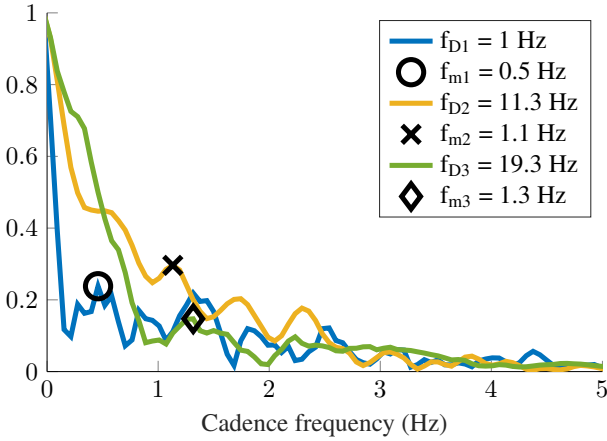
Fig. 4: Cadence frequencies represented by the circle, cross and diamond markers, corresponding to the Doppler bins 1 Hz, 11.3 Hz and 19.3 Hz respectively.
