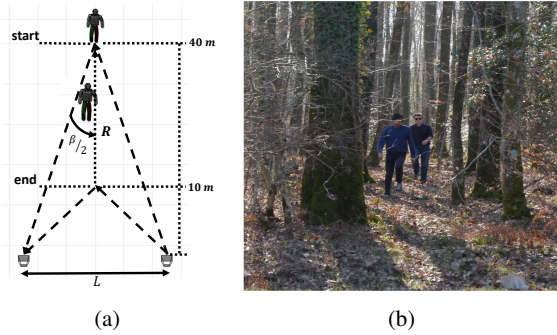
Fig. 1: Measurement setup: (a) parameters of the bistatic configuration, (b) couple of persons moving among the trees.
