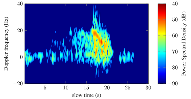
Fig. 2: Spectrogram of a couple of persons walking and running among the trees at 1 GHz.
