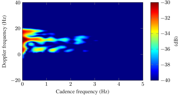
Fig. 3: Cadence frequency diagram of a couple of persons walking and running among the trees at 1 GHz.
