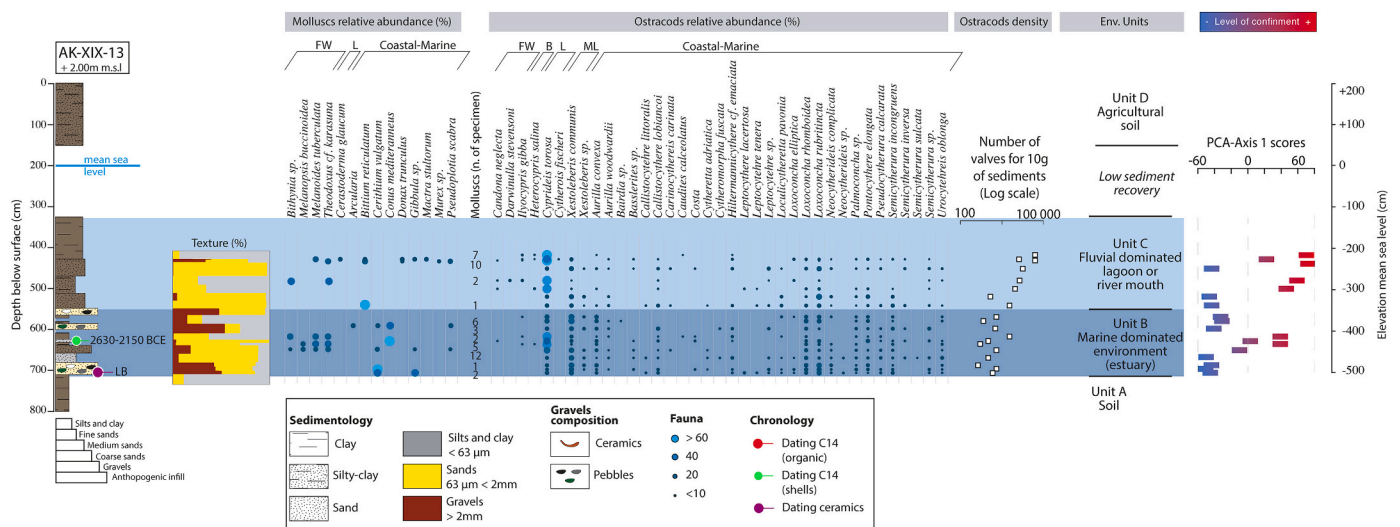
Fig. 5. Sediment texture and faunal analysis of core AK-XIX-13. Four different environmental units were identified. As with AK-XIX-16 (Fig. 4), the succession of the units shows the development of a lagoon – over a coastal environment – due to the progradation of the coast and the river-mouth. See Fig. 3 for location of the core.
