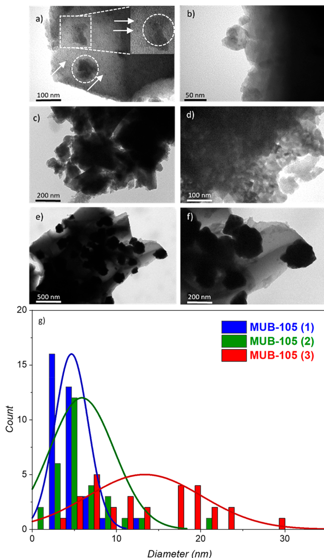
Figure 4. Investigation at the mesoscopic length scale through TEM. (a, b) MUB-105(1), (c, d) MUB-105(2), and (e, f) MUB-105(3), (g) Nb 2 O 5 primary crystallite size deconvolution using the ImageJ program. White circles show Nb 2 O 5 aggregated crystals and white arrows show isolated crystals. The continuous gray scale represents the siliceous continuous phase. An average of 5 μm 2 has been investigated for each samples.
