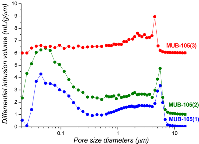
Figure 2. Pore size distribution obtained through mercury porosimetry. MUB-105(1) blue dots, MUB-105(2) green dots, and MUB-105(3) red dots. For the sake of clarity, the MUB-105(2) and the MUB-105(3) curves have been offset by 1.0 and 6.0 mL/(g μm), respectively.
