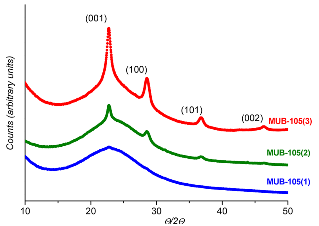
Figure 7. WAXS investigation. MUB-105(1) blue dots, MUB-105(2) green dots, and MUB-105(3) red dots. Main diffraction peaks of the \text{Nb}_2\text{O}_5 pseudohexagonal TT- \text{Nb}_2\text{O}_5 (JCPDS 28-317).
