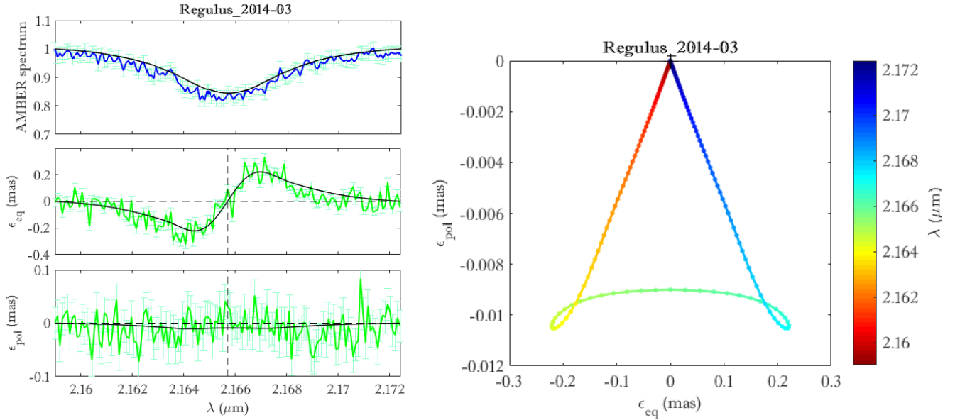
Figure 11. Comparison between observations and the best MCMC minimization parameters model, through the two photocentre displacements ( \epsilon_{\alpha}, \epsilon_{\delta} ) and spectrum, Top: over the AMBER spectrum of Regulus in the \text{Br}\gamma line. Bottom: The equatorial-polar photocentre displacements ( \epsilon_{\text{eq}}, \epsilon_{\text{pol}} ). Right: Best modeling of vectorial photocentre displacement ( \epsilon_{\text{pol}} = f(\epsilon_{\text{eq}}) ).
