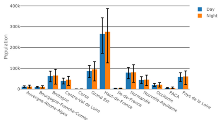
Figure 6. Number of people exposed to WT sound level above 30 dBA, by region. Error bars account for the uncertainty of +/-1 standard deviation on the Harmonoise sound level estimate.
