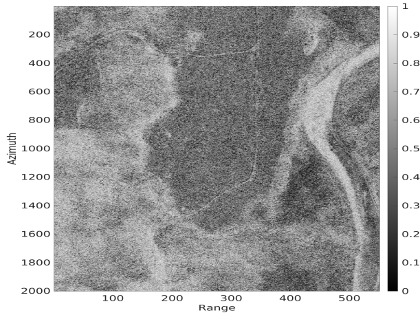
Fig. 3: Temporal Entropy
