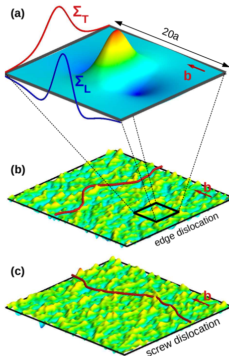
FIG. 1: Anisotropy of shear stress autocorrelations:
