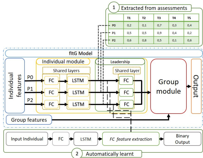
Figure 2: Architecture to integrate the 2 approaches from the Representation Based Leadership family into the fitG model: i) the Extracted from Assessments is using leadership scores, ii) the Automatically Learnt is generated using a deep learning model. Both of them are integrated into the cohesion model in the individual module using a shared FC layer after the concatenation.
