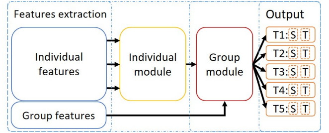
Figure 1: Architecture of the fitG model to predict the dynamics of Social and Task cohesion. It is composed of 4 modules (i.e., Features extraction, Individual, Group, and Output modules). The dynamics of cohesion for the Social (S) and Task (T) dimensions are predicted for the 5 tasks (T1 to T5) in a multilabel setting.
