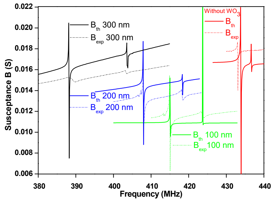
Figure 6. Theoretical and experimental responses of quartz (YX)/45°/10° resonators for different \text{WO}_3 thicknesses: 100 nm, 200 nm, and 300 nm.
