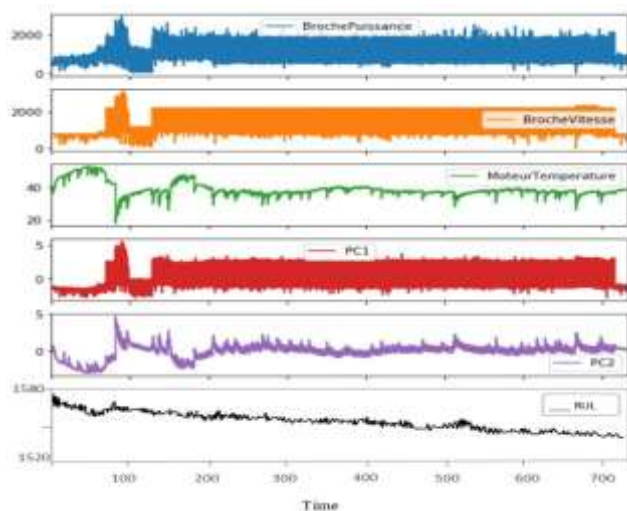
Fig. 7. PCA visualization regarding component state
