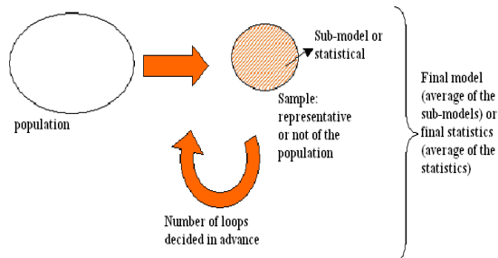
Fig. 1: Principle of the method of the Bootstrap
