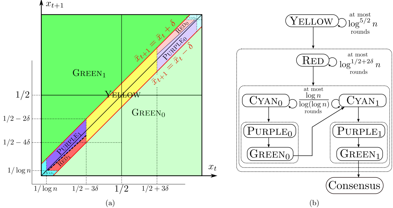
Figure 1: (a) Partitioning the state space into domains. The x-axis (resp., y-axis) represents the proportion of agents with opinion 1 in round t (resp., t + 1 ). The thick dashed line at the frontier between PURPLE 1 and RED 1 is defined by x_{t+1} = (1 - \lambda_n)x_t . (b) Sketch of the proof of Theorem 1. All transitions are w.p. at least 1 - 1/n^{\Omega(1)} . The numbers next to the self-loops indicate that the process stays in the corresponding domain for this number of rounds w.p. at least 1 - 1/n^{\Omega(1)} . The source is assumed to have opinion 1.
