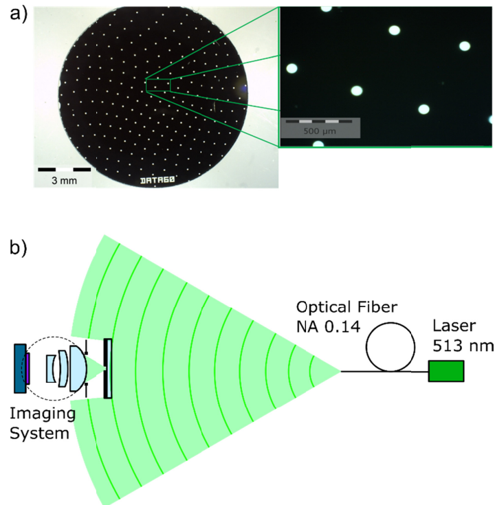
Fig. 3. Experimental set-up for self-focusing effect validation: (a) pictures of a sinusoidal periodic apertures distribution mask, (b) set-up description.
