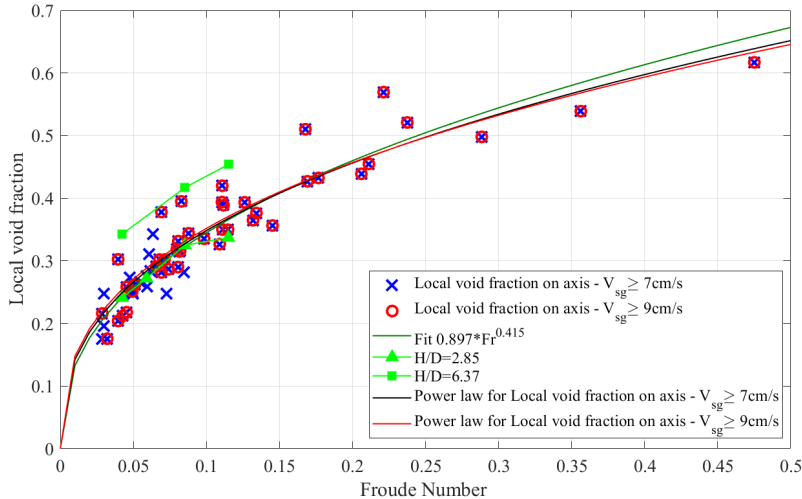
Figure 30: Correlation between the local void fraction on the axis of the column and the Froude number Fr = V_{sg}/(gD)^{1/2} for all experiments quoted in Tables 1 and 2. Measurements performed for 1.3 \leq H/D \leq 12 . To illustrate the impact of H/D , the data with closed symbols correspond to measurements in the D=0.4\text{m} column performed at moderate ( H/D=2.85 , triangles) and at large ( H/D=6.37 , squares) distances from injection.
