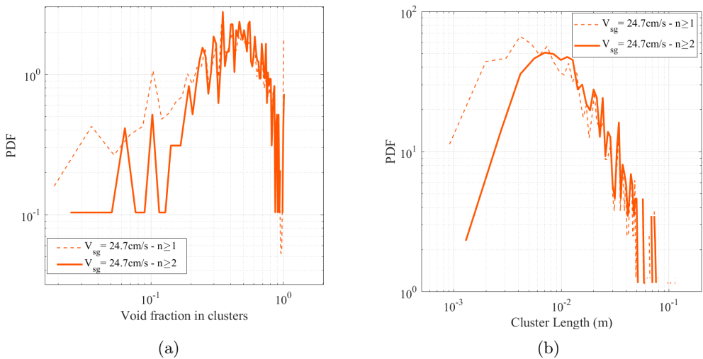
Figure 18: Comparisons of the pdfs of void fraction in clusters (a) and of clusters lengths (b) when the minimum number of bubbles is set to 1 or to 2. Measurements performed in a D = 0.4\text{m} column, on the column axis at H/D = 3.625 and V_{sg} = 24.7\text{cm/s} .
