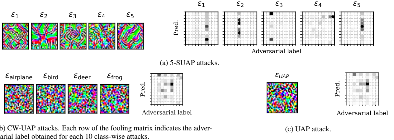
Figure 2: \ell_\infty -based attacks on CIFAR-10. In the fooling matrices, labels range {airplane, automobile, bird, cat, deer, dog, frog, horse, ship, truck} from top to bottom and left to right.
