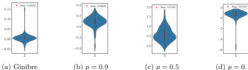
Fig. 14: Violin plots of Z obtained using \widehat{S}_{BI} across A = 50 samples from the Ginibre and the corresponding independent thinning with retaining probability p . The computation is done using structure_factor .
