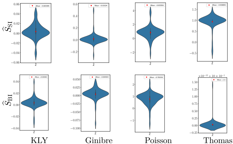
Fig. 12: Violin plots of Z across 50 samples from the KLY, Ginibre, Poisson, and Thomas point process using \hat{S}_{SI} (first line) and \hat{S}_{BI} (last line). The computation is done using structure_factor
