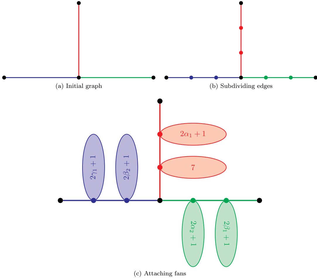
Figure 2: Illustration of the reduction in the proof of Theorem 2.3, for d = 3 . (a) represents the neighbourhood of a vertex in H , its three incident edges being assigned colour 1 (red), 2 (green), and 3 (blue) by \phi . In the first step of the reduction (b), all edges are subdivided d - 1 = 2 times. Then, in the second step (c), the subdivided vertices resulting from the subdivision of a red edge are being attached a 7-fan and a (2\alpha_1 + 1) -fan, respectively, the subdivided vertices resulting from the subdivision of a green edge are being attached a (2\alpha_2 + 1) -fan and a (2\beta_1 + 1) -fan, respectively, and the subdivided vertices resulting from the subdivision of a blue edge are being attached a (2\beta_2 + 1) -fan and a (2\gamma_1 + 1) -fan, respectively. Ellipses represent k -fans on the indicated values of k .
