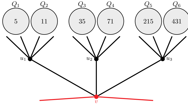
Figure 1: Attaching a k -fan (in black) at a degree-2 vertex v (in red). Circles represent cliques on the indicated numbers of vertices. Here, k = 5 for simplicity. Q_1 is a k -clique, thus a 5-clique, while Q_2 is a (2k + 1) -clique, thus an 11-clique. Setting n_1 = d(u_1) = 17 , Q_3 is a (2n_1 + 1) -clique, thus a 35-clique, while Q_4 is a (2(2n_1 + 1) + 1) -clique, thus a 71-clique. Setting n_2 = d(u_2) = 107 , Q_5 is a (2n_2 + 1) -clique, thus a 215-clique, while Q_6 is a (2(2n_2 + 1) + 1) -clique, thus a 431-clique. Note that, after the attachment, v is of degree 5.
