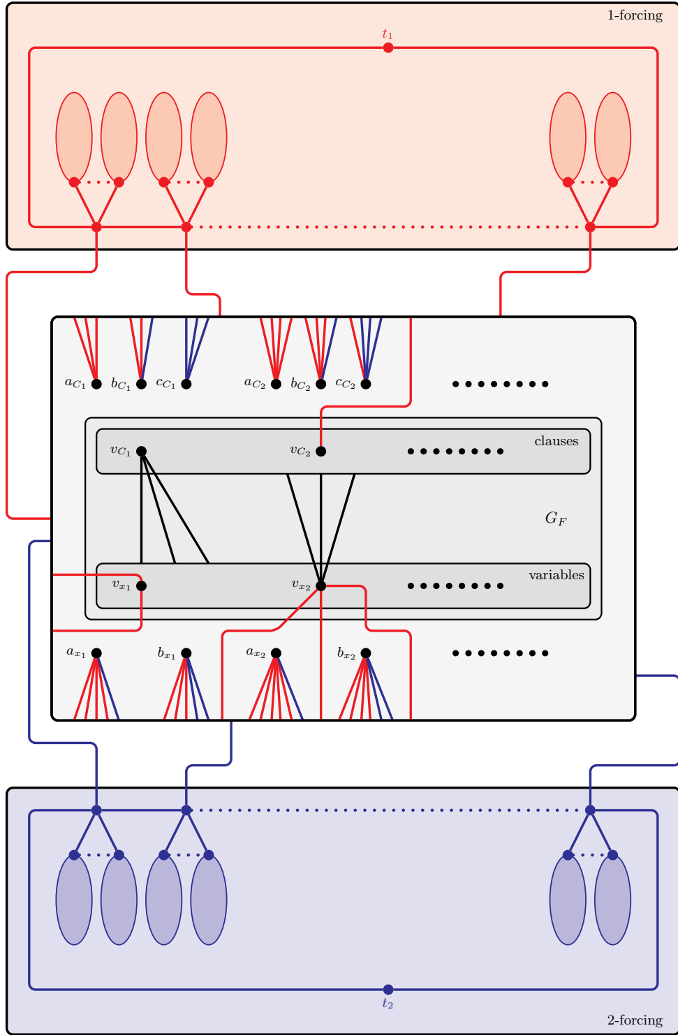
Figure 3: Part of the reduction in the proof of Theorem 3.3. The connected component containing w and all cliques attached to it are not represented. Red edges are 1-edges by any m -irregular 2-labelling, while blue edges are 2-edges. Ellipses represent cliques. Note that in each of the sets \{v_{C_1}, a_{C_1}, b_{C_1}, c_{C_1}\} , \{v_{C_2}, a_{C_2}, b_{C_2}, c_{C_2}\} , \{v_{x_1}, a_{x_1}, b_{x_1}\} , and \{v_{x_2}, a_{x_2}, b_{x_2}\} , all vertices have the same degree due to incident 1-edges and 2-edges, and that any two of these sets contain vertices with distinct degrees. For every i \in \{1, 2\} , due to a_{C_i}, b_{C_i} , and c_{C_i} , note that, in an m -irregular 2-labelling, it must be that one formula edge incident to v_{C_i} is assigned label 1 while the other two are assigned label 2. Likewise, for every i \in \{1, 2\} , due to a_{x_i} and b_{x_i} , all formula edges incident to v_{x_i} must be assigned the same label.
