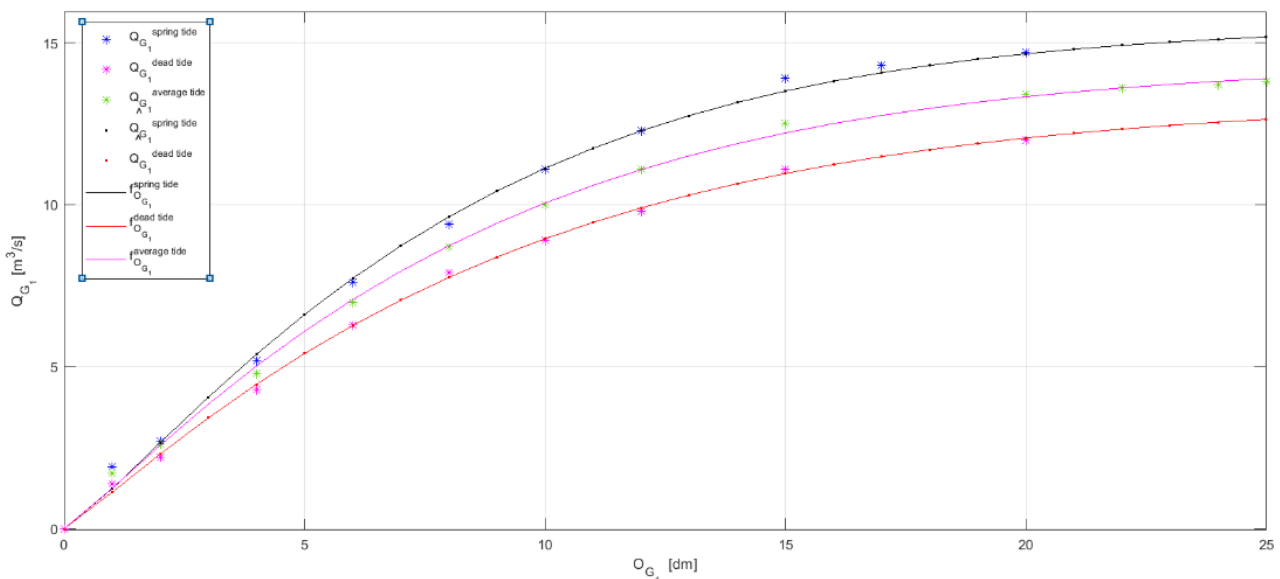
Figure 4: Estimated discharge Q_G [m³/s] function of gate opening O_G [dm] according to the type of tide, with the points given by managers (star), and the estimated points (dot).
