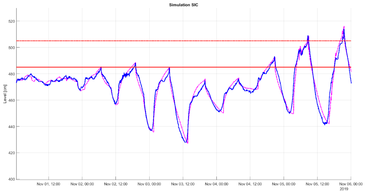
Figure 7: Level of the Calais canal from November 1 st to November 6 th , 2019, in blue (real measurement), in magenta (simulated one), by considering a loss of flow and delay for the gates.
