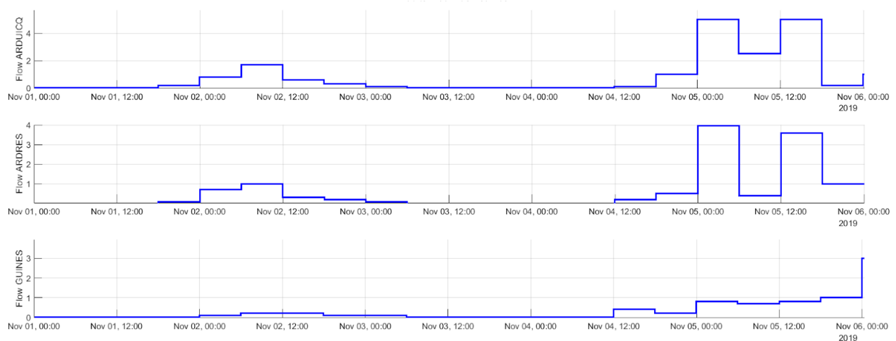
Figure 10: Estimated flows based on the model with loss of flow and delay, from a) Ardrucq canal, b) Ardres canal, c) Guines canal.
