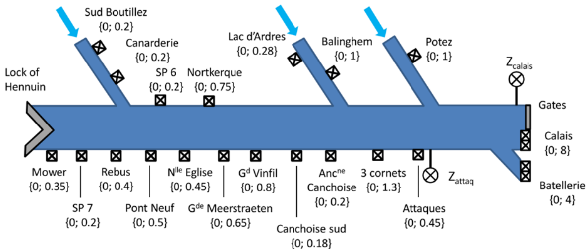
Figure 2: Schematic view of the Calais canal.
