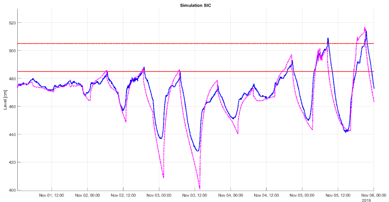
Figure 6: Level of the Calais canal from November 1 st to November 6 th , 2019, in blue (real measurement), in magenta (simulated one), by considering an average flow for the gates.
