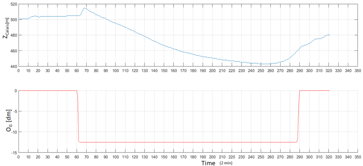
Figure 5: a) Level in Calais Z_{calais} , b) gate opening O_G for November 6 th , 2019, time in sample of 2 minutes.
