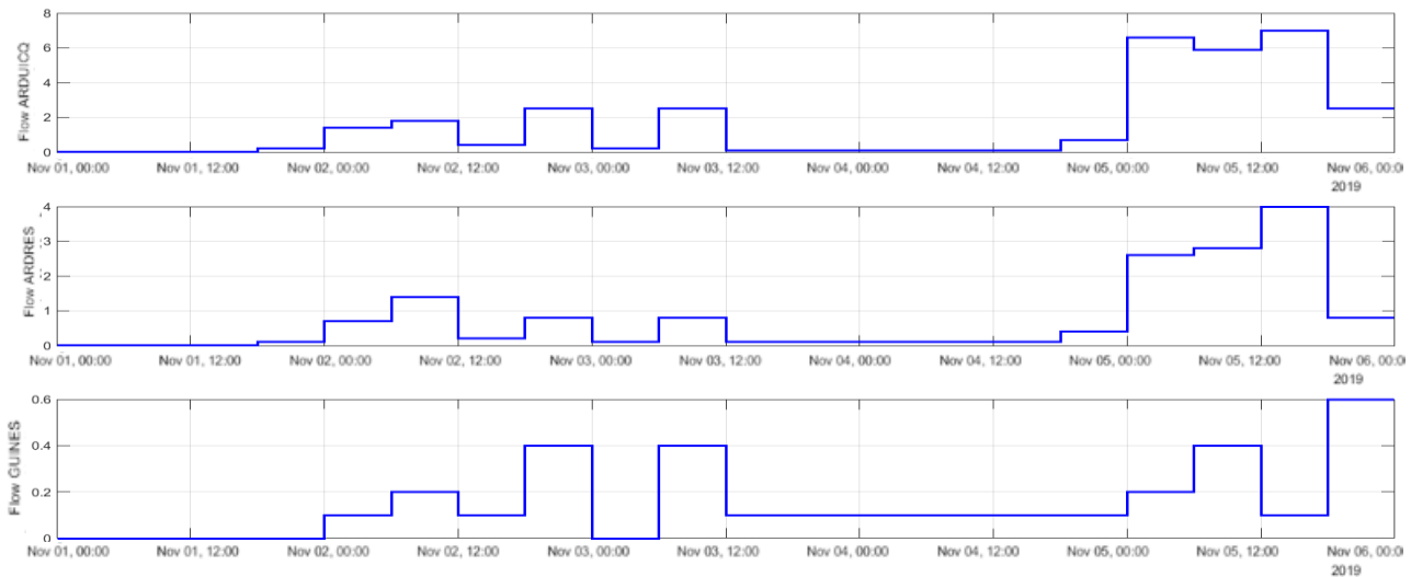
Figure 9: Estimated flows based on the model with average flow, from a) Ardrucq canal, b) Ardres canal, c) Guines canal.
