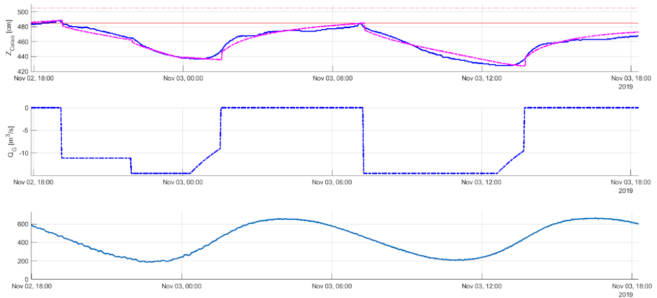
Figure 8: a) Level of the Calais canal from November 2 st to November 3 rd , 2019, in blue (real measurement), in magenta (simulated one), b) the flow of the gate QG with a loss of flow and delay, c) the sea level.
