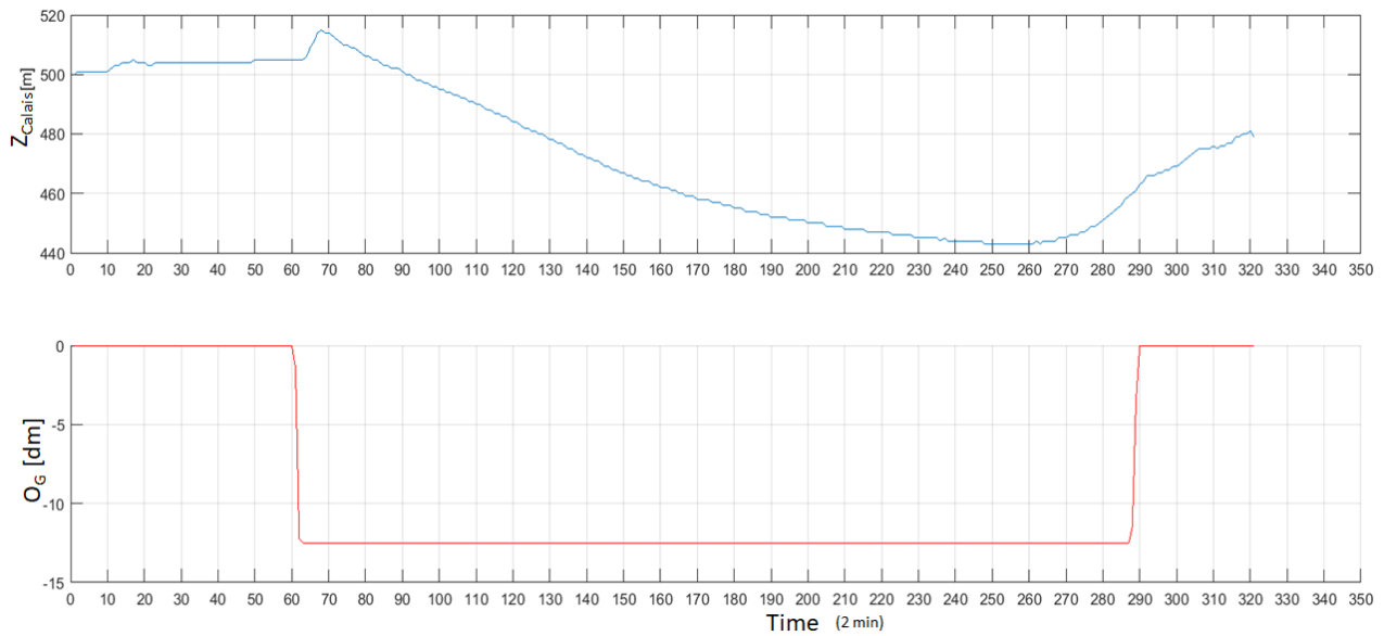
Figure 5: a) Level in Calais Z_{\text{Calais}} , b) gate opening O_G for November 6 th , 2019, time in sample of 2 minutes.
