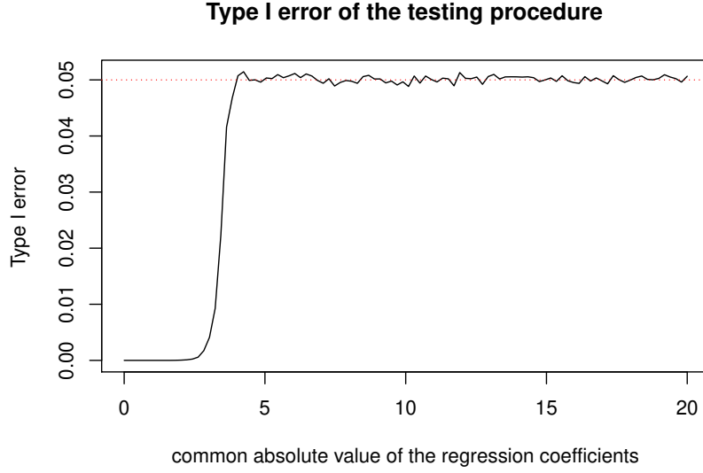
Figure 3: This picture reports the type I error (on the y-axis) of the testing procedure as a function of \|\beta\|_\infty (on the x-axis). Each point from this plot is obtained via 100000 simulations. Theoretically, under the null hypothesis and when \|\beta\|_\infty is infinitely large, the type I error is controlled at level \alpha = 0.05 . This curve corroborates this fact. Moreover, it seems the type I error is controlled at level \alpha = 0.05 for any value of \|\beta\|_\infty \geq 0 .
