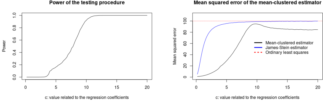
Figure 4: The picture on the left reports the power (on the y-axis) of the testing procedure as a function of the value c given in (7). One may observe that, approximately, the power is 1 when c > 10 and the power is smaller than 1 when c < 10 . The picture on the right reports the mean squared error as a function of c of the mean-clustered estimator, the ordinary least squared estimator and the James-Stein estimator. Note that the mean-clustered estimator outperforms both the ordinary least squares estimator as well as the James-Stein estimator. One may observe that the curve is increasing when c < 10 and is slightly decreasing when c > 10 . Thus, the mean squared error starts to decrease when the power of the procedure is 1, namely when components of the OWL estimator cannot be all equal in absolute value.
