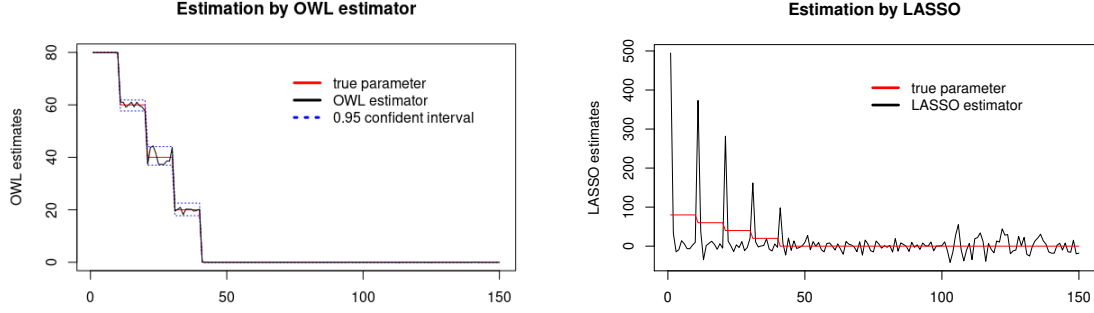
Figure 6: The picture on the left illustrates performance of OWL estimator for recovering \beta as described in (8). Note that the number of non-null clusters is k = 4 and thus according to Figure 5 the noiseless recovery condition does not hold thus OWL estimator cannot recover exactly the pattern of \beta . However, the accessibility occurs thus OWL estimator may separate clusters (see Tardivel et al. (2021) for additional details). Indeed, for each i \in \{1, \dots, 150\} the probability that \hat{\beta}_i lies into the blue band is 0.95 thus OWL estimator is a quite accurate estimator of \beta . The right picture illustrates that LASSO fails to recover \beta in this setting.
