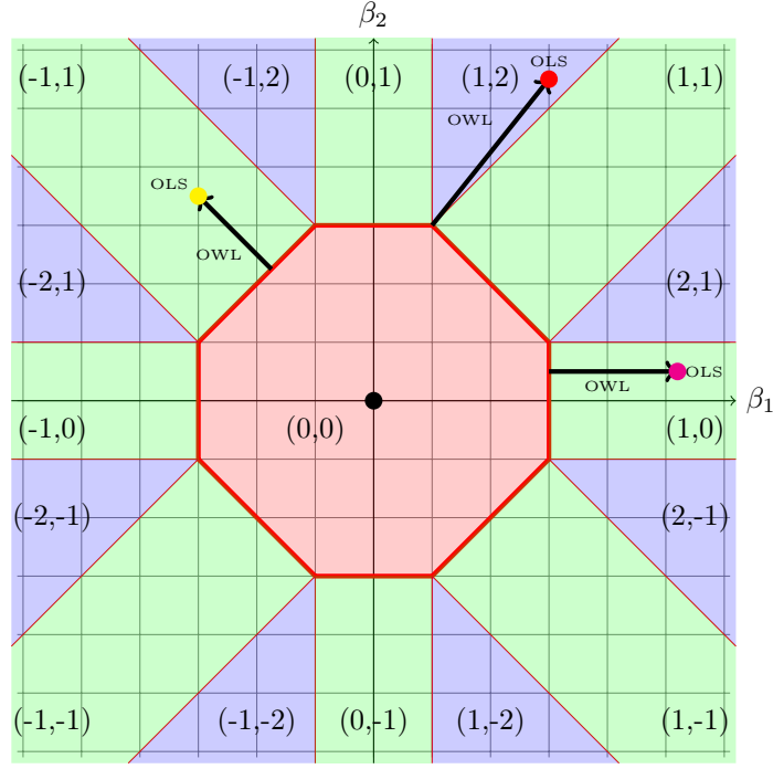
Figure 1: This figure represents the OWL estimator \hat{\beta} (illustrated by black arrows) depending on the localization of \hat{\beta}^{\text{ols}} in the particular case where X'X = I , w = (3, 1) and \gamma = 1 . When \hat{\beta}^{\text{ols}} is the pink point located on the area labelled by (1, 0) then the first component of \hat{\beta} is positive and the second is null. When \hat{\beta}^{\text{ols}} is the yellow point located on the area labelled by (-1, 1) then both components of \hat{\beta} are equal in absolute value; the first component is negative and the second is positive. When \hat{\beta}^{\text{ols}} is the red point located on the area labelled by (1, 2) then both components of \hat{\beta} are positive and the first component is smaller than the second. The red polytope is the signed permutahedron P^\pm(w) and labels \mathcal{P}_2^{\text{owl}} = \{(0, 0), \pm(1, 0), \pm(0, 1), \pm(1, 1), \pm(1, -1), \pm(2, 1), \pm(2, -1), \pm(1, 2), \pm(1, -2)\} associated to areas of this figure correspond to OWL patterns in \mathbb{R}^2 .
