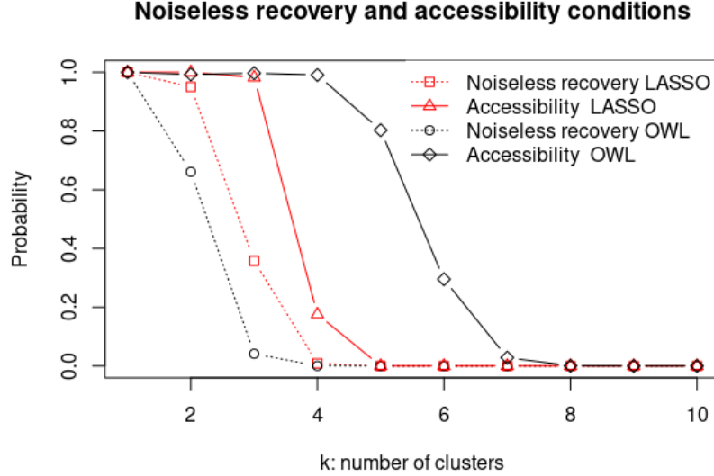
Figure 5: When X \in \mathbb{R}^{50 \times 150} is a random matrix described in 1), these curves provide the probability that the noiseless recovery condition occurs and the probability that the accessibility condition occurs as a function of k (the number of clusters) for both LASSO and OWL estimator when \rho = 0.99 . One may notice that noiseless recovery curves are below accessibility curves; these observations comply with theoretical property: noiseless recovery condition implies accessibility condition. Note that accessibility curves for OWL estimator are above accessibility curves for LASSO. This suggest that, potentially, OWL estimator is a better estimator than LASSO for pattern recovery in the particular setting where some columns are almost equal.
