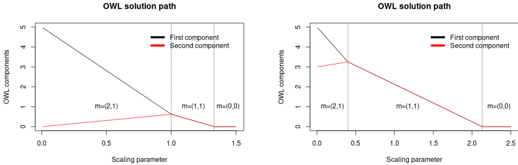
Figure 2: On the left the signal is \beta = (5, 0) . Based on this figure one may observe that the pattern of \beta cannot be recovered by OWL estimator in the noiseless case (despite the fact that \hat{\beta}(\gamma) tends to \beta when \gamma tends to 0). Indeed, for \gamma \in (0, \gamma_1) (where \gamma_1 \approx 1 ) we have \text{p}_{\text{owl}}(\hat{\beta}(\gamma)) = (2, 1) ; when \gamma \in [\gamma_1, \gamma_2) (where \gamma_2 \approx 1.33 ) we have \text{p}_{\text{owl}}(\hat{\beta}(\gamma)) = (1, 1) and when \gamma > \gamma_2 then \hat{\beta}(\gamma) = 0 . Consequently, for every \gamma > 0 we have \text{p}_{\text{owl}}(\hat{\beta}(\gamma)) \neq \text{p}_{\text{owl}}(\beta) = (1, 0) . On the right the signal is \bar{\beta} = (5, 3) . Based on this figure one may observe that \text{p}_{\text{owl}}(\bar{\beta}) is recovered by OWL estimator in the noiseless case. Indeed, for \gamma \in (0, \gamma_1) (where \gamma_1 \approx 0.4 ) we have \text{p}_{\text{owl}}(\hat{\beta}(\gamma)) = (2, 1) = \text{p}_{\text{owl}}(\bar{\beta}) .
