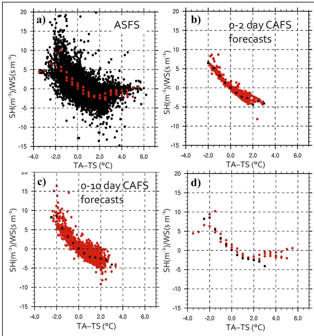
Figure 21. An example of process-based model evaluation. (a) Ten-minute average observations of scaled sensible heat fluxes (2-m sensible heat flux divided by 2-m wind speed, in units of \text{W s m}^{-3} ) relative to near-surface stratification (2-m air temperature minus skin temperature, in ^{\circ}\text{C} ) from 3 ASFS flux stations (black) and values binned for each flux station individually in intervals of 0.5^{\circ}\text{C} (red). (b) Same as (a) but from 6-hourly output from 0–2 day forecasts from Coupled Arctic Forecast System (CAFS). (c) Same as (b) but using the CAFS 0–10 day forecasts to show that the model is not drifting into a different state. (d) Binned values from (a) and (c) to compare the observations (red) and model (black) forecasts more closely. ASFS = Atmospheric Surface Flux Stations. DOI: https://doi.org/10.1525/elementa.2021.00060.f21
