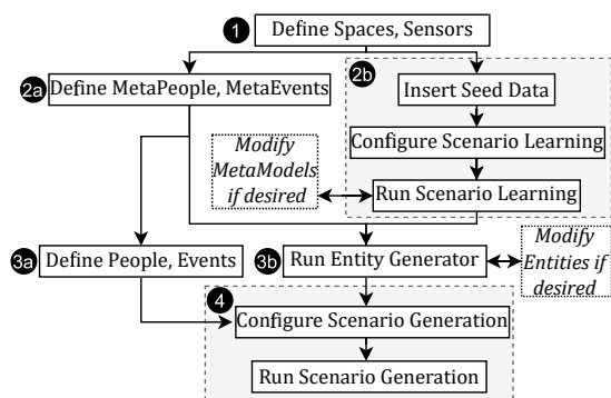
Fig. 1: SmartSPEC workflow.
