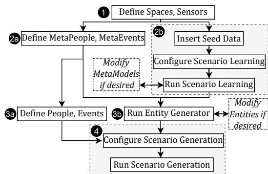
Fig. 1: SmartSPEC workflow.
