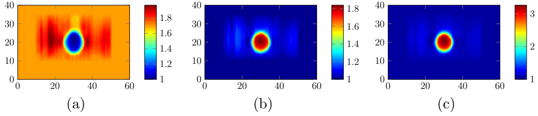
Figure 8: Relative shear modulus maps obtained with the 3D simulations, for media characterized by inclusion-to-background shear modulus ratios of (a) 4/9 (case #4), (b) 16/9 (case #5), and (c) 27/9 (case #6). Axes are in mm.
