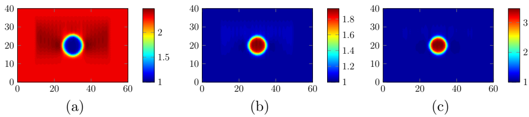
Figure 7: Relative shear modulus maps obtained with the plane stress simulations, for media characterized by inclusion-to-background shear modulus ratios of (a) 4/9 (case #1), (b) 16/9 (case #2), and (c) 27/9 (case #3). Axes are in mm.
