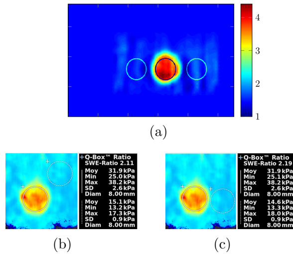
Figure 11: Illustration of region selection for modulus ratio computation with the scanned area containing a single inclusion in the breast elastography phantom (case #9). Regions selected in the map reconstructed with (a) our method, and (b) and (c) the Aixplorer.
