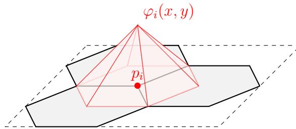
Figure 2: Graph of the test function \varphi_i .
