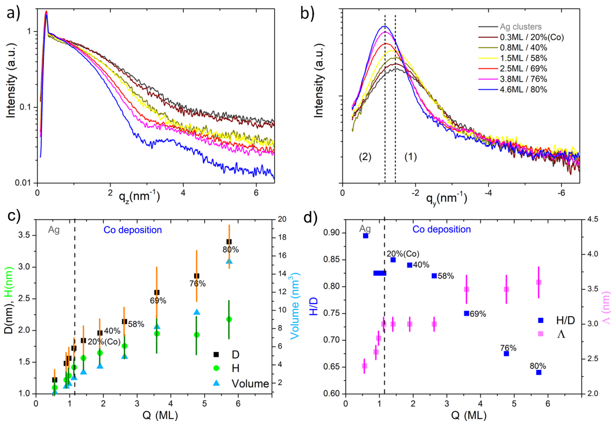
Fig. 3 GISAXS spectra during Co deposition: a) normalized on the intensity of the Yoneda peak in the q_z direction and b) raw in the q_y direction. Evolution of the average parameters (vertical bars correspond to the width \sigma of the Gaussian distributions): c) diameter D , height H and volume V , and d) aspect ratio ( H/D ) of the particles and interparticle distance ( \Delta ) relative to the quantity of matter Q in equivalent thickness in monolayers (ML) of atoms.
