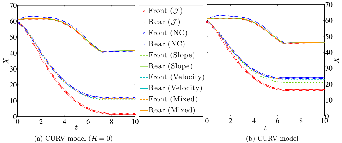
Figure 19: Test 3: Evolution in time of the front and rear flow positions calculated with the CURV models with and without correction \mathcal{J} ( \delta_0 = 30^\circ ).
