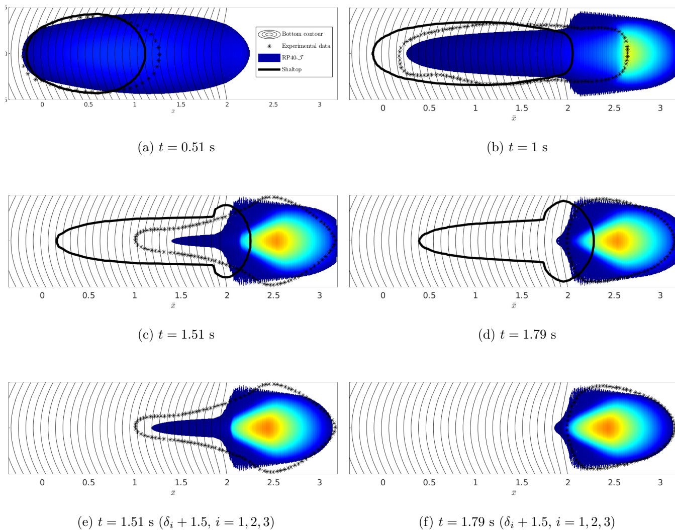
Figure 33: Test 8: Comparison of the solution of the SHALTOP model (black line) with experimental data and with those of the RP40- \mathcal{J} model (Pouliquen friction law, L = 3.9 mm, \gamma = 10^{-3} , \delta_1 = 21^{\text{circ}} , \delta_2 = 30.7^{\circ} , \delta_3 = 22.2^{\circ} ). Figures (e) and (f) correspond to the solution of the RP40- \mathcal{J} model adding 1.5 degrees to \delta_1 , \delta_2 and \delta_3 .
