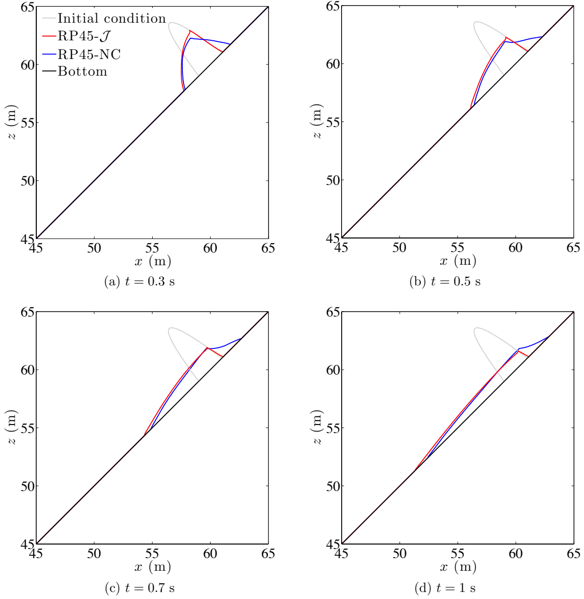
Figure 8: Test 1: Comparison between the RP45-NC and RP45- \mathcal{J} models ( \delta_0 = 37^\circ ).
