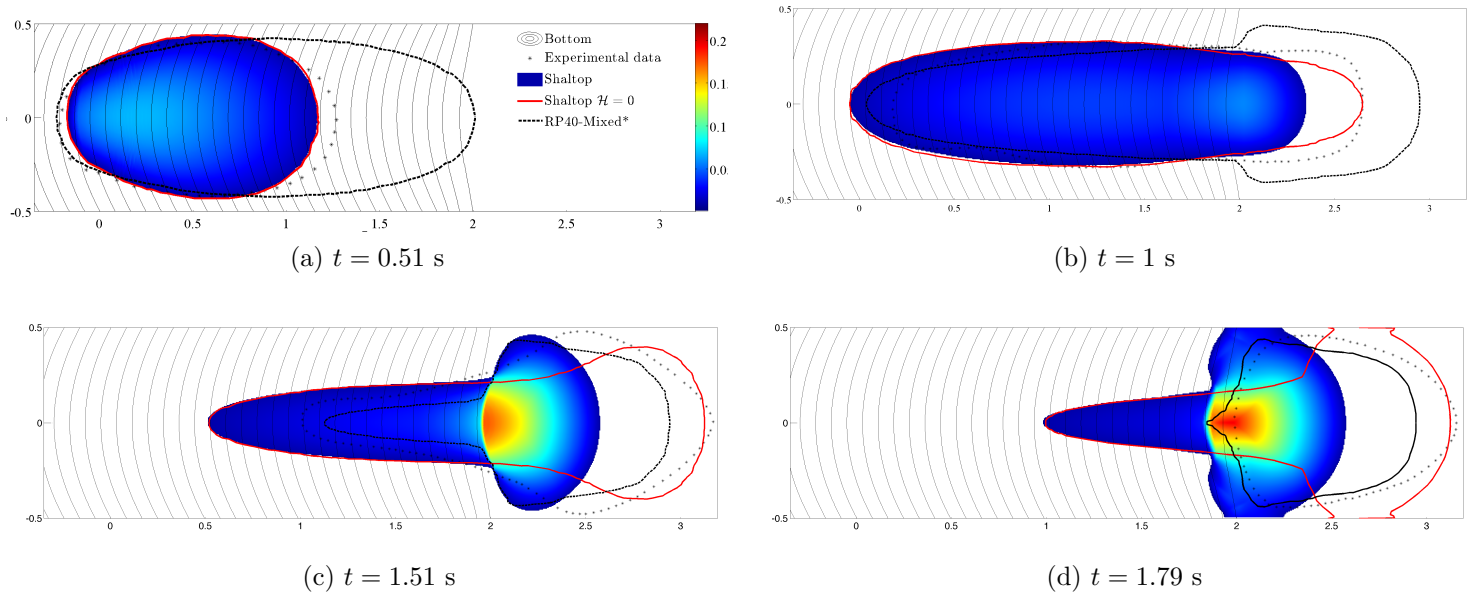
Figure 32: Test 8: Comparison of the solution of the SHALTOP model with experimental data and with those of the SHALTOP ( \mathcal{H} = 0 ) and RP40-Mixed* models (Coulomb friction law, \delta_0 = 30^\circ ).
