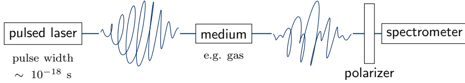
Figure 1: Simplified experimental setup for measuring ultrashort (e.g. a few attoseconds 10^{-18} s) electromagnetic polarized pulses. Inspired by [20, 21].
