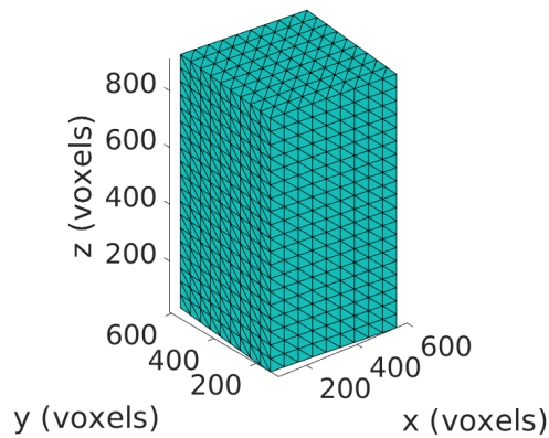
Figure 5. Mesh in the reference configuration consisting of 9,234 T4 elements. The size of the analyzed region of interest is 480 \times 470 \times 893 \text{ vx} (or 19.8 \times 19.4 \times 38.4 \text{ mm} )
