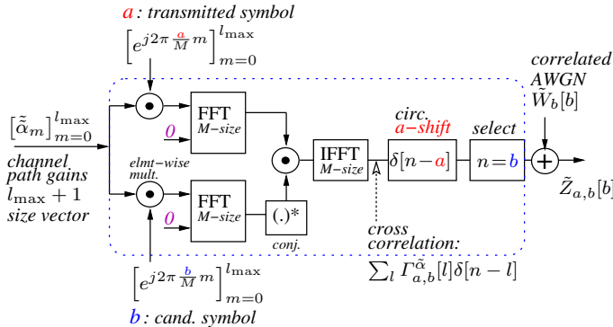
Fig. 6. Equivalent system model (39) for the MF receiver and by considering the received signal approximation given in (18).
