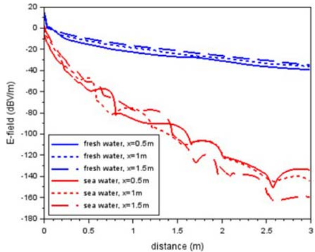
Figure 2. Simulated electric field at 10 MHz as a function of the distance to the radiating wire in water for various conductivities (from 0.04 S/m to 4 S/m). The radiating wire is 20 m long and the excitation port (power = 1 W) is placed in the middle.
