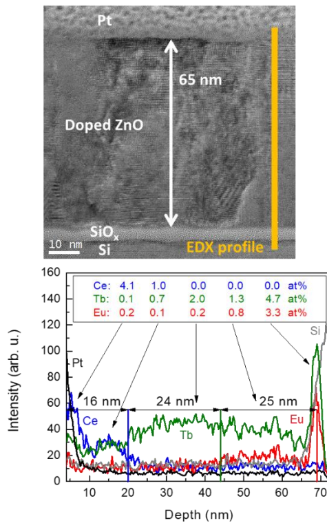
Figure 2. (a) TEM image corresponding to the deposited sample containing the ZnO:Ce/ZnO:Tb/ZnO:Eu,Tb stack, being the total stack thickness measured to be ~65 nm. (b) EDX depth profiles for Pt, Si, Ce, Tb and Eu, obtained through 120 points measured along the 75 nm indicated with a vertical a line in (a).
