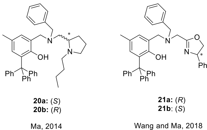
Fig. 7 Ligands developed for magnesium coordination
