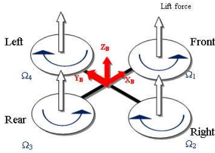
Fig. 1: Quadrotor schematic.
