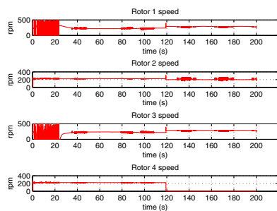
Fig. 7: Rotor speeds of the quadrotor (Damage of fourth rotor).
