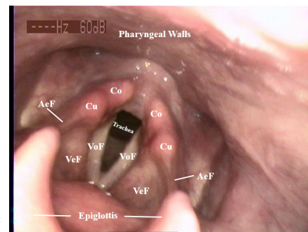
(b) Epilaryngeal Structures: Vocal Folds (VoF), Ventricular Folds (VeF), Aryepiglottic Folds (AeF), Cuneiform Cartilages (Cu) and Corniculate Cartilages (Co)
