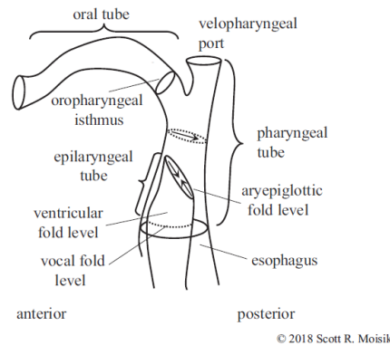
(a) Laryngeal Sphincters
