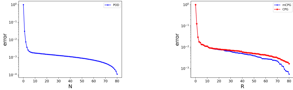
Figure 11: Hertz test-case: projection errors for the POD, CPG and mCPG algorithms. Left: POD. Right: CPG and mCPG.
