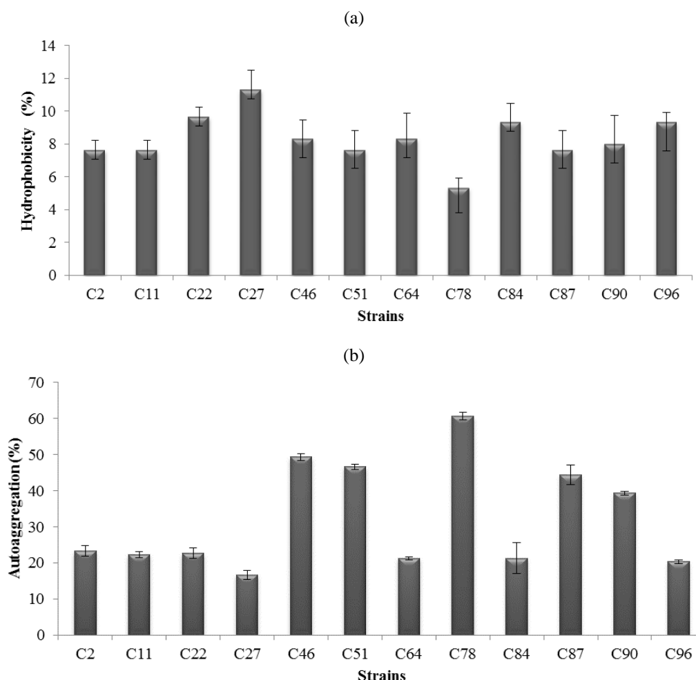
Figure 2. Percentage of hydrophobicity (a) and auto-aggregation (b) of lactobacilli strains isolated from goat milk.
